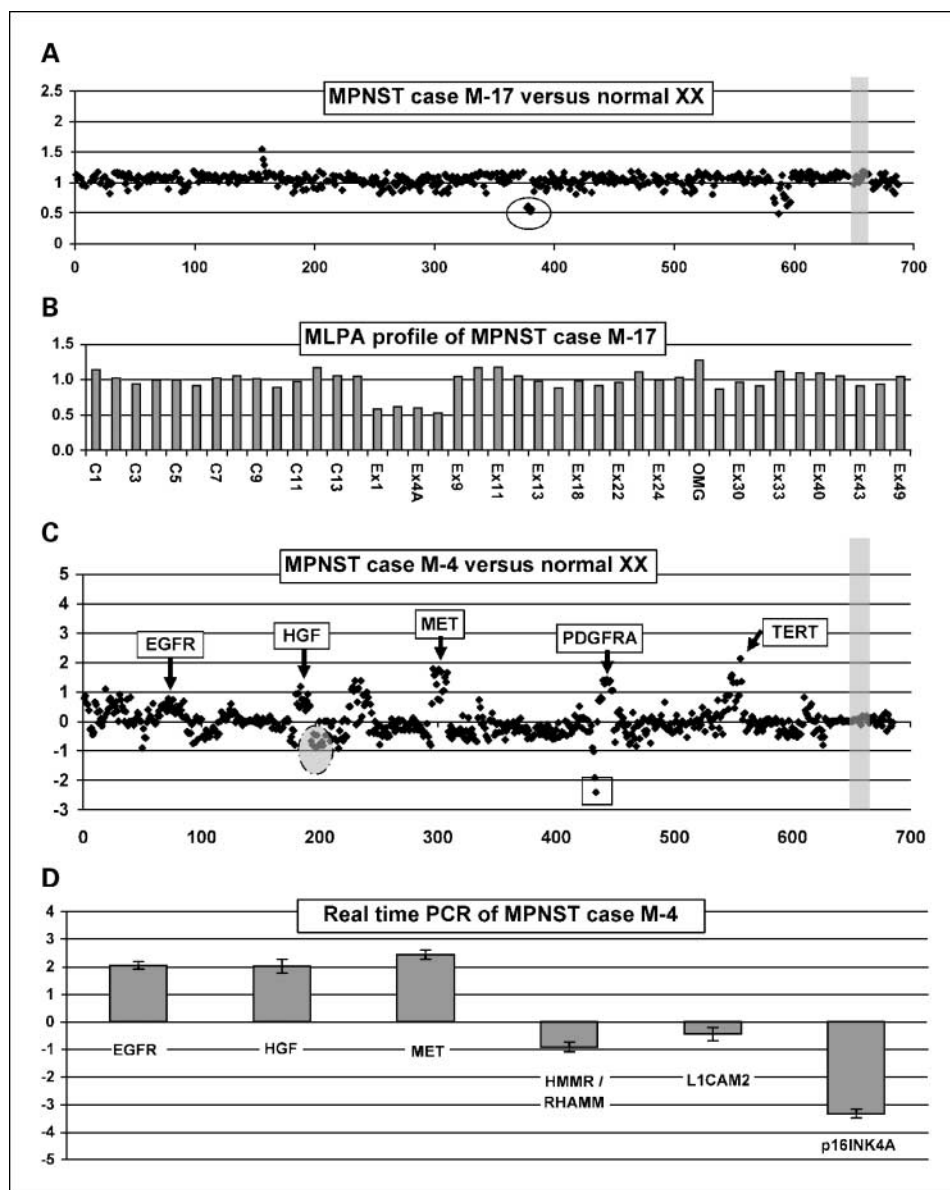
Fig. 4. Confirmation of array CGH data by MLPA and real-time PCR. A , array CGH profile of DNA derived from MPNST sample M-17. The intragenic deletion in the NF1 gene was detected by five measurement points (ID 376-380; -0.83 \pm 0.03 ) that span exons 2 through 7. B , the MLPA analysis of M-17 sample for DNA copy number alterations in the NF1 gene revealed an intragenic deletion spanning exons 1 through 6 ( 0.58 \pm 0.04 ). Probes C1-C14, autosomal control probes. C , array CGH analysis of MPNST case M-4. Shaded oval, one copy deletion of the HMMR/RHAMM gene ( -0.66 \pm 0.07 ); rectangle, biallelic loss of p16INK4A/CDKN2A gene ( -1.64 \pm 0.71 ). The copy number gains are indicated for EGFR ( 0.50 \pm 0.10 ), HGF ( 0.74 \pm 0.26 ), MET ( 1.5 \pm 0.51 ), PDGFRA ( 1.26 \pm 0.22 ), and TERT ( 0.65 \pm 0.20 ) genes. D , validation of DNA copy number changes in MPNST case M-4 using real-time PCR. Y-axis, \log_2 ratios of gene copy number and the SD values across the triplicate measurements. The suboptimal level for deletion of the L1CAM2 deletion by real-time PCR may be explained by the polyploid nature of the MPNST.
